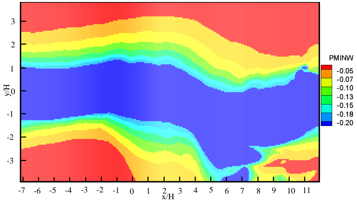
Figure 6.18 Minimum pressure on 2D ridge surface for (V_0/V_t=4) .
