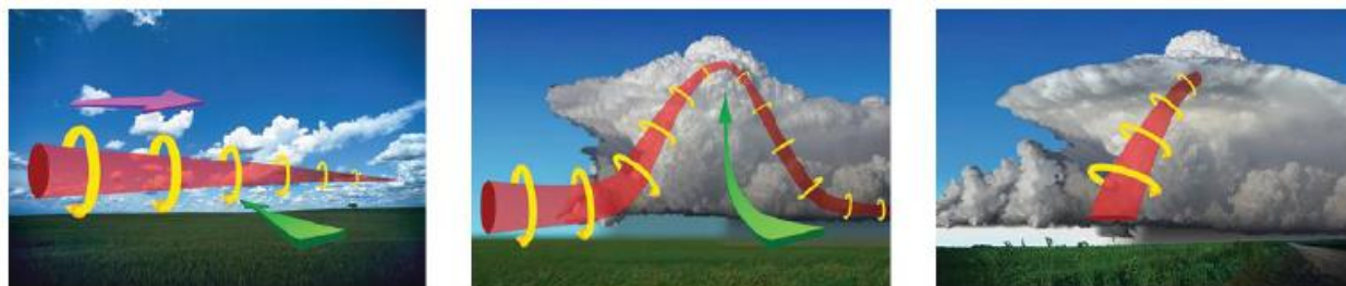
Figure 2.1 Tornado Formation in Tornado Alley taken from Tornadoes (2012).
