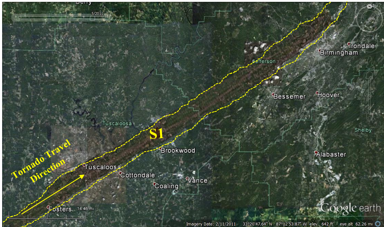
Figure 4.10 The tornado path of Tuscaloosa-2011 tornado show the investigated site (the bright color area is the damaged area path).
