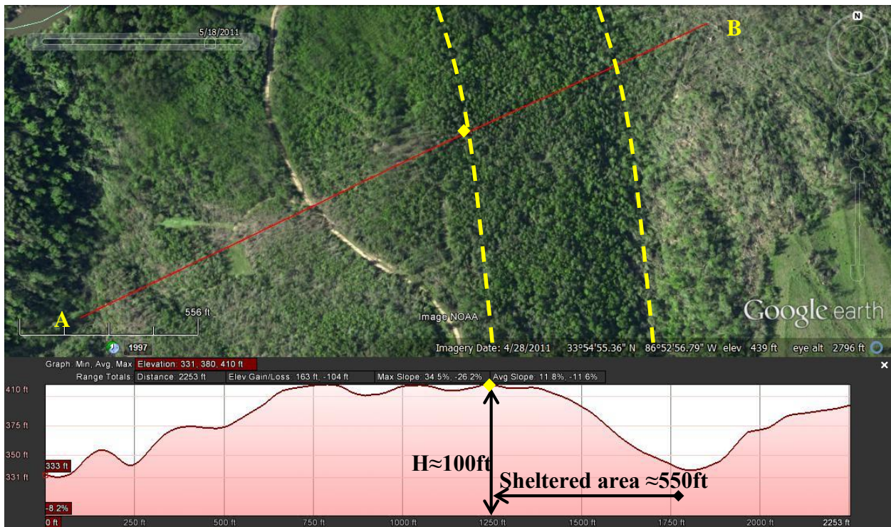
Figure 4.7 Elevation profile along the hill (H3), the protected zone is 5.5H.
